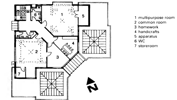
6 First floor → 5
